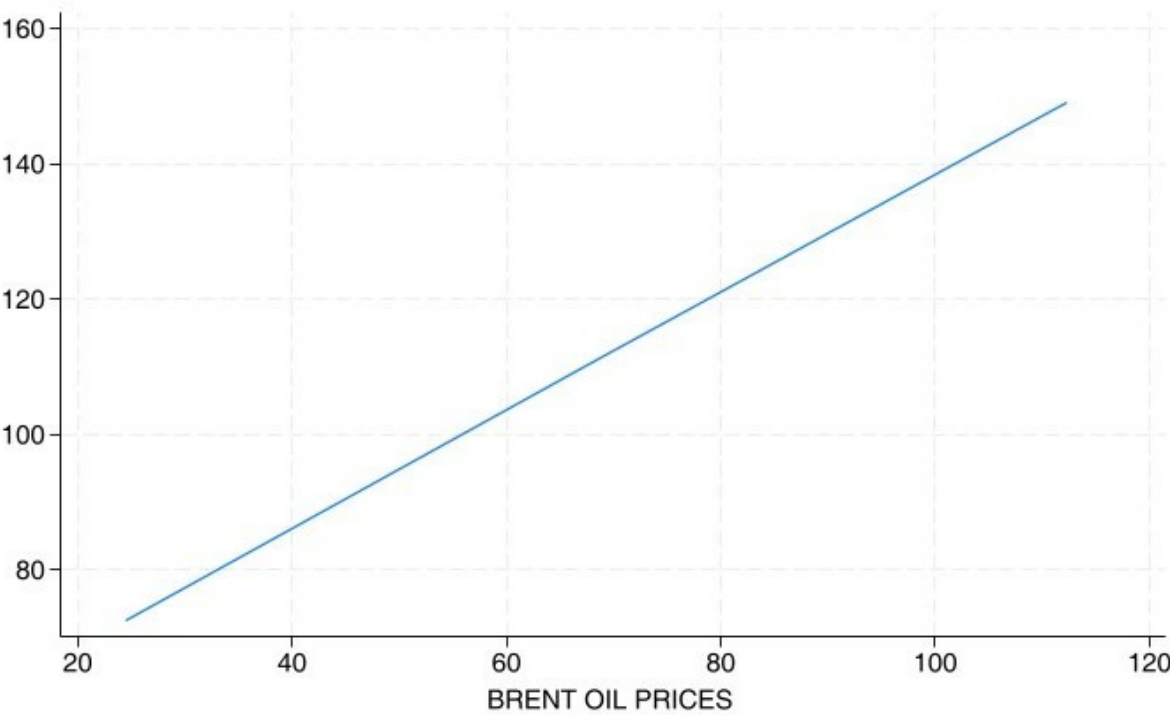
Figure 4: CFPI vs Brent Oil Prices
