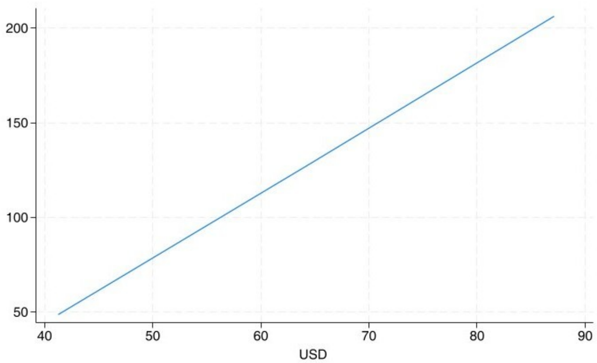
Figure 2: CFPI vs USD/INR exchange rates
