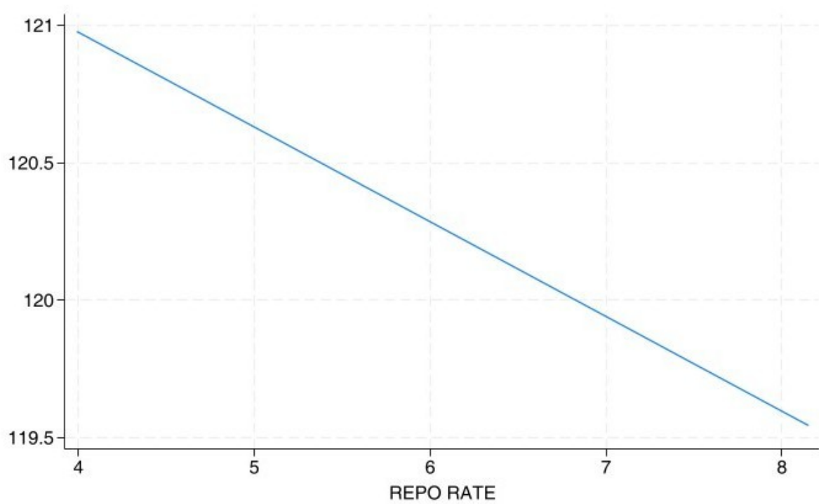
Figure 3: CFPI vs Repo Rate
