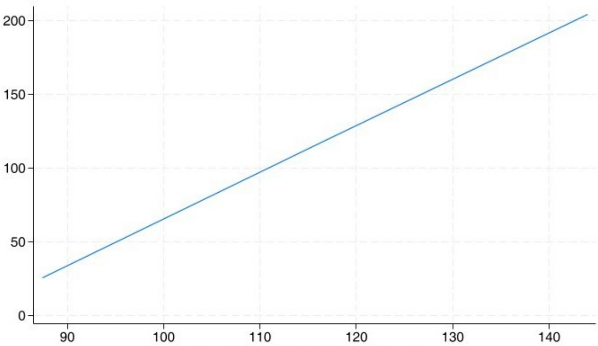
Figure 5: CFPI vs Fertilizer WPI
